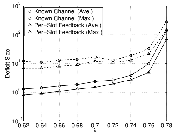
Fig. 5. Comparison of the average and maximum deficit size for different channel models
