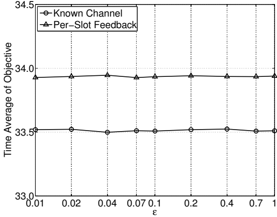
Fig. 6. Average objective for different values of \epsilon
