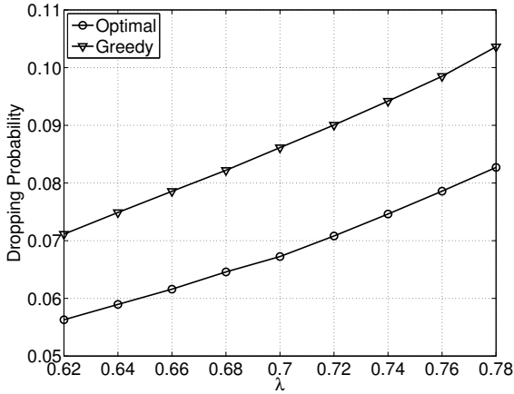
Fig. 2. Comparison of dropping probability for a greedy approximation
