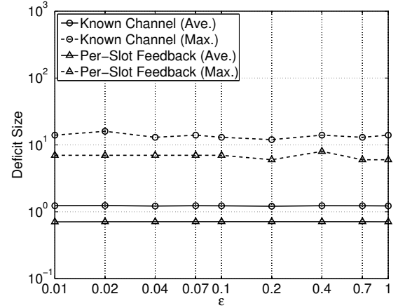
Fig. 7. Deficit size for the different values of \epsilon
