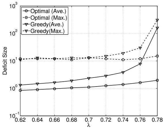
Fig. 3. Comparison of the average and maximum deficit size for a greedy approximation
