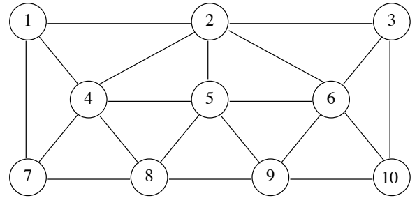
Fig. 1. Interference graph used in the simulations
