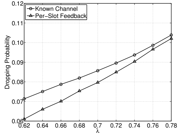
Fig. 4. Comparison of dropping probability for different channel models
