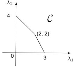
Fig. 2. The capacity region \mathcal{C}
