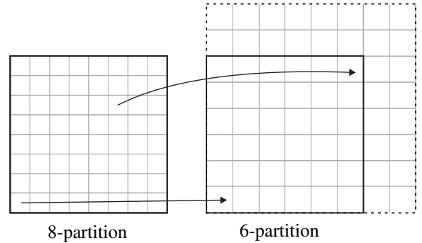
Figure 5. Constructing a 6-partition from the original 8-partition.
