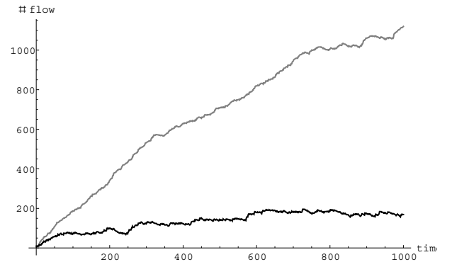
Figure 3. Evolution of the total number of flows for MaxWeight scheduling (gray) and an interval-based randomized scheduler (black), respectively.
